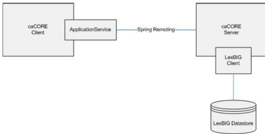
Figure 4.5 - DLB Architecture
