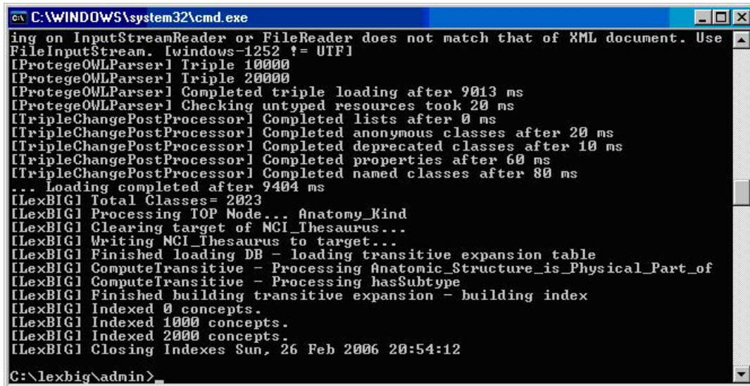
Figure 3 - Displays the successful load of the sample vocabulary file.
